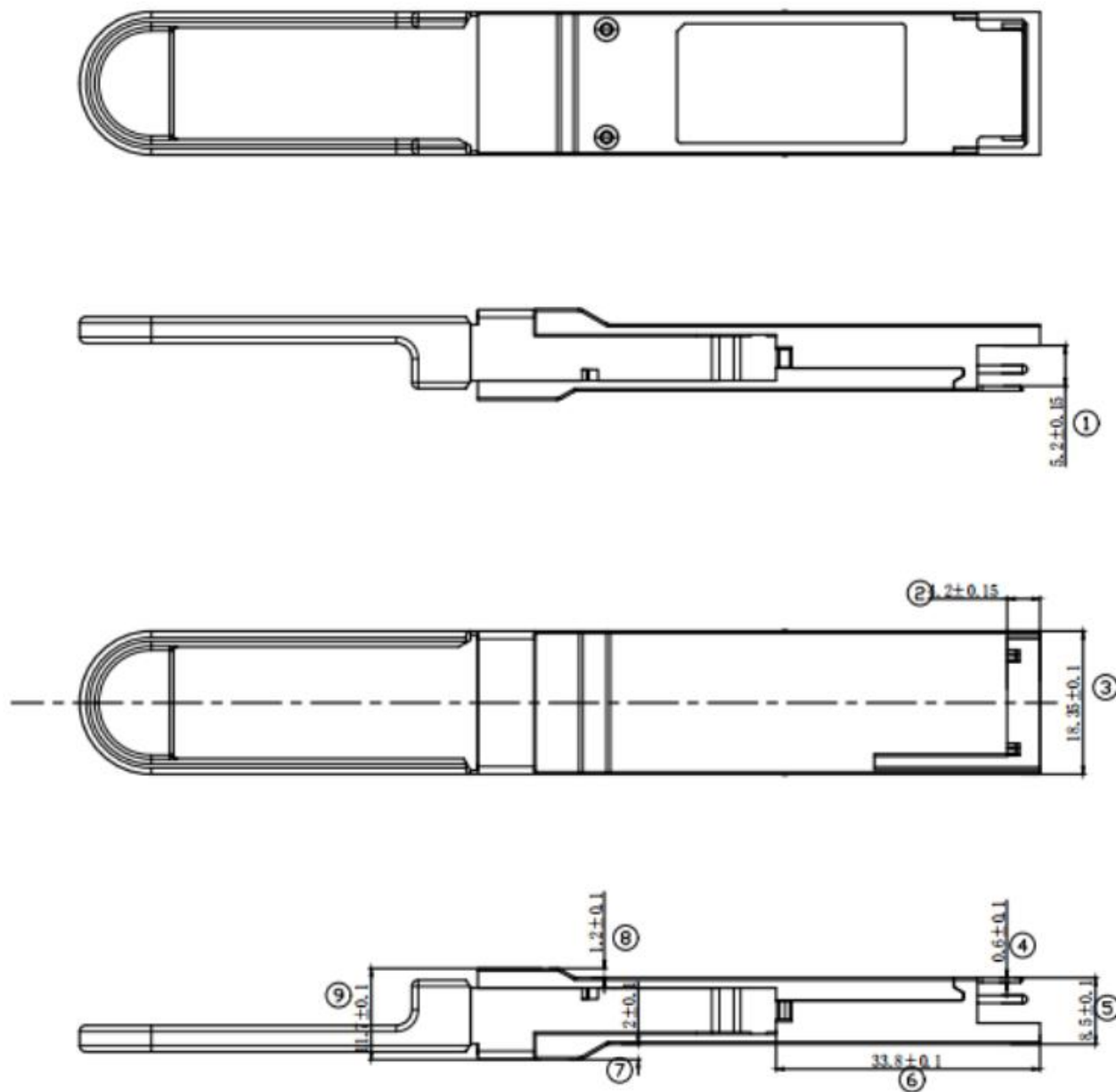
Figure 7, Mechanical Dimensions
