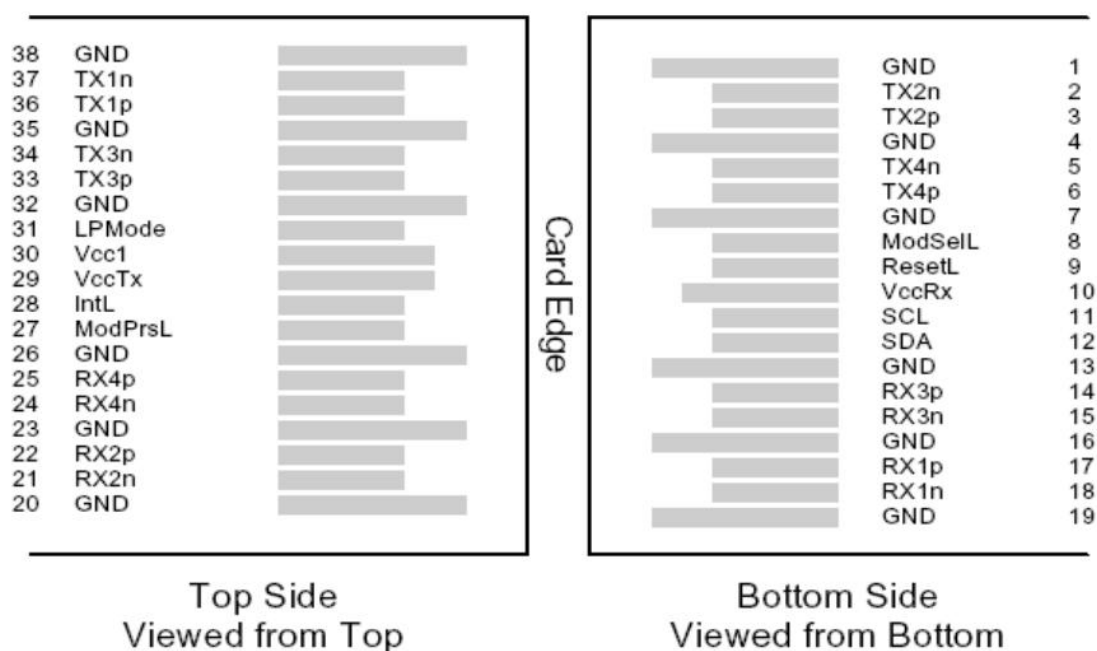
Figure 2. Host PCB QSFP+ pad assignment top view and Names
