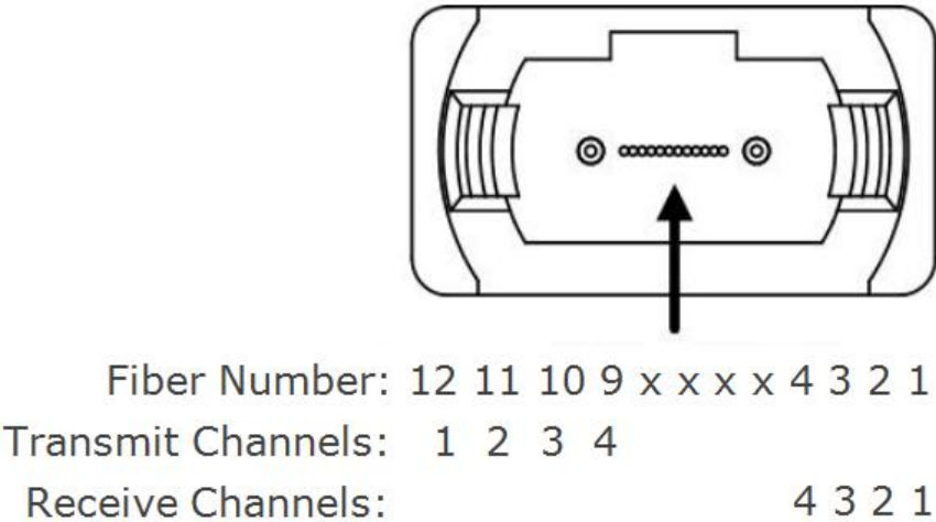
Figure 3. QSFP+ Optical Receptacle and Channel Orientation
