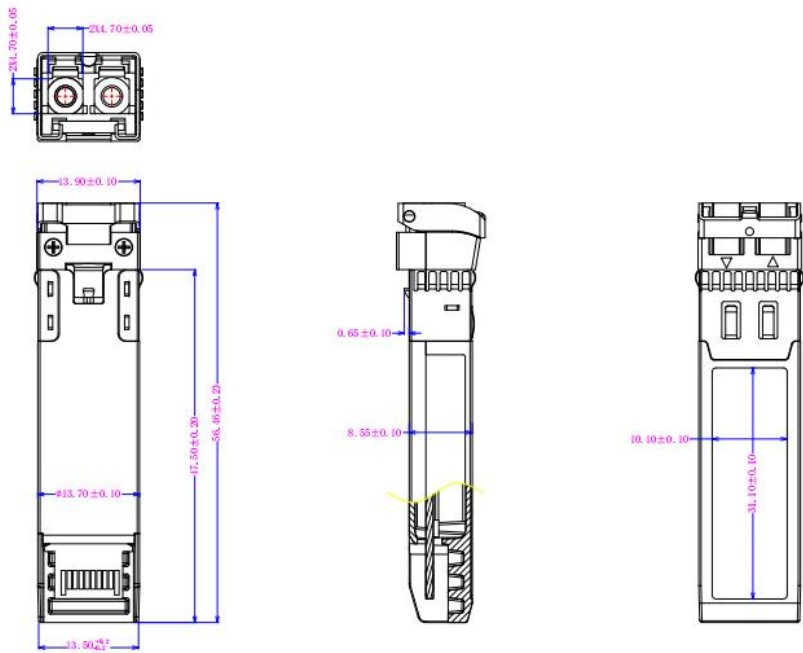
Figure 5, Mechanical Dimensions
