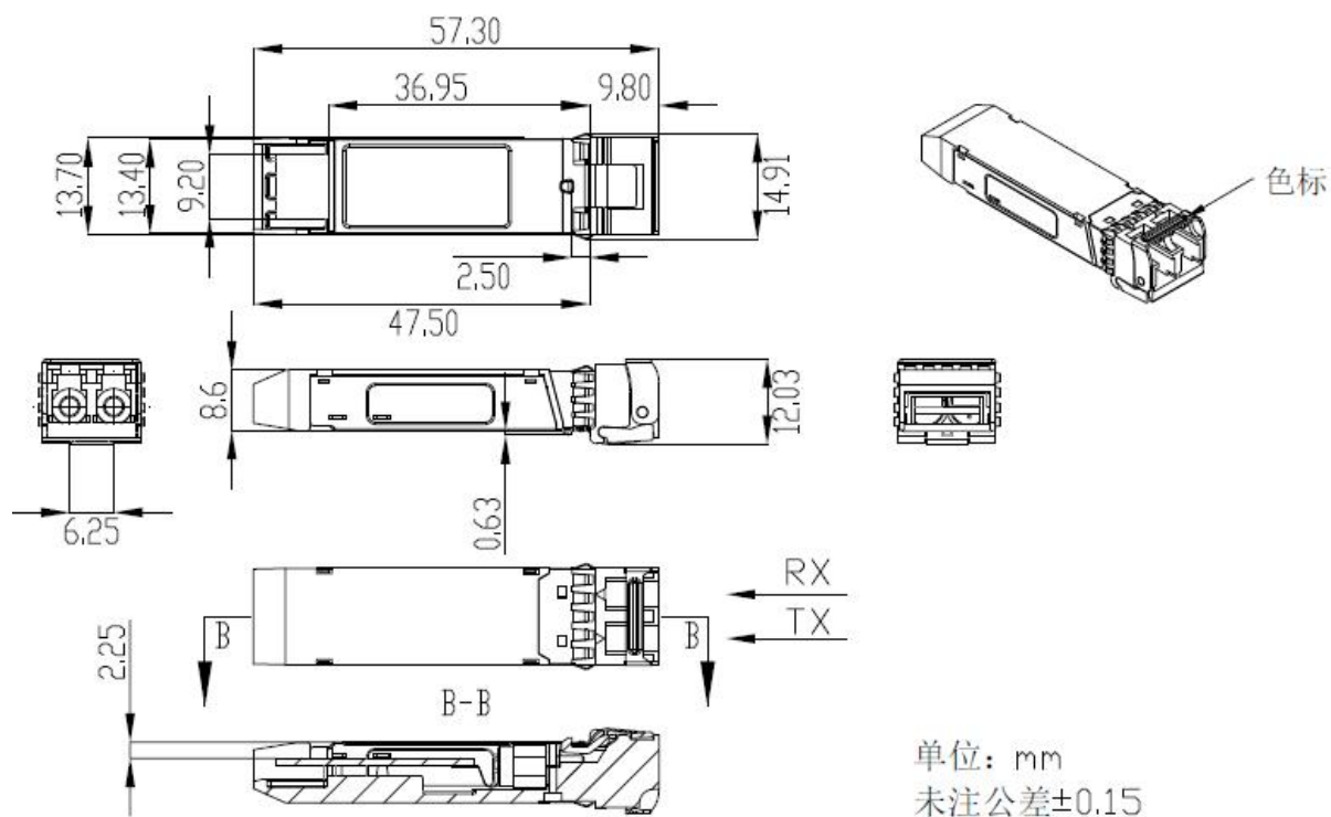
Figure 5, Mechanical Dimensions
