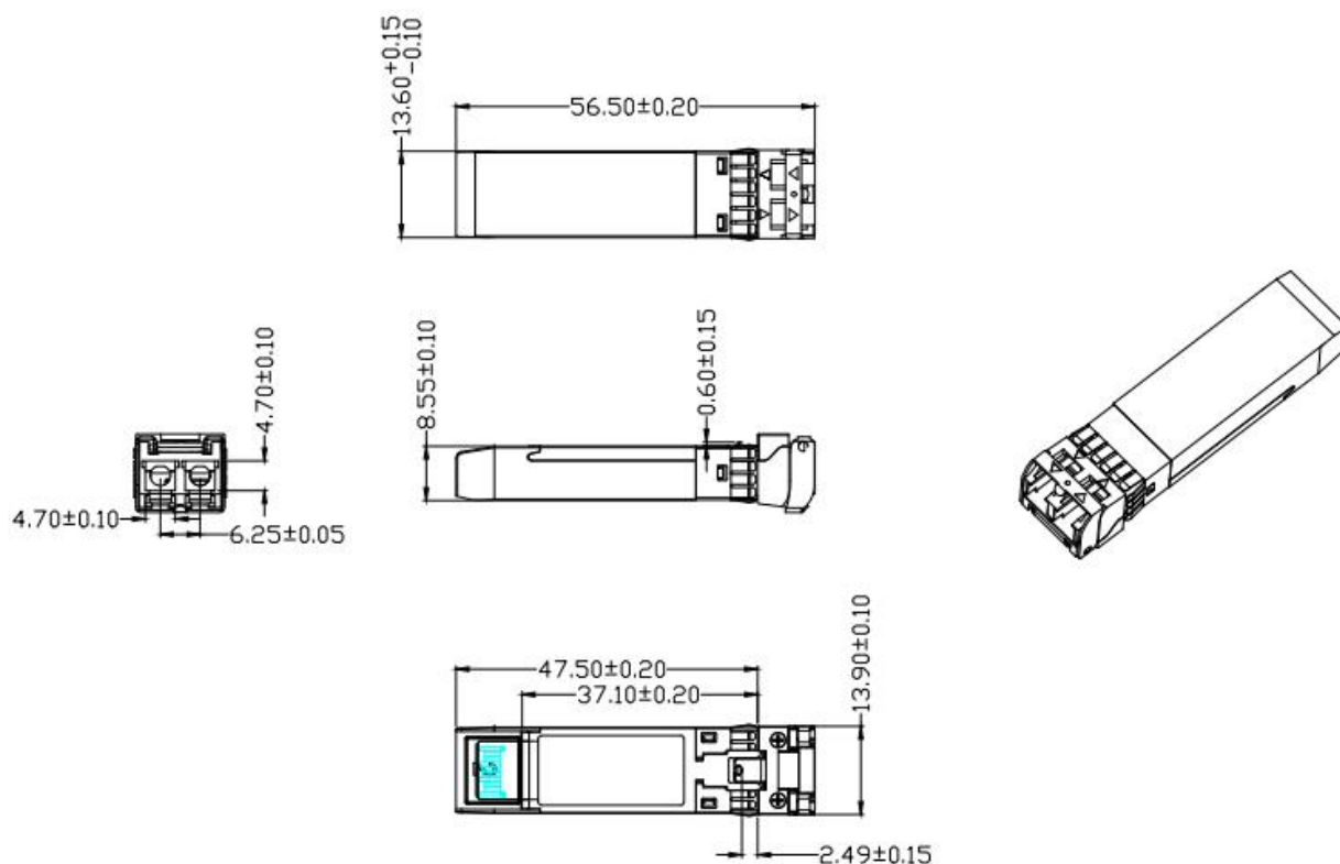
Figure 5, Mechanical Dimensions
