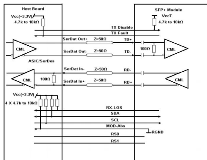
Figure 4, Recommended Interface Circuit
