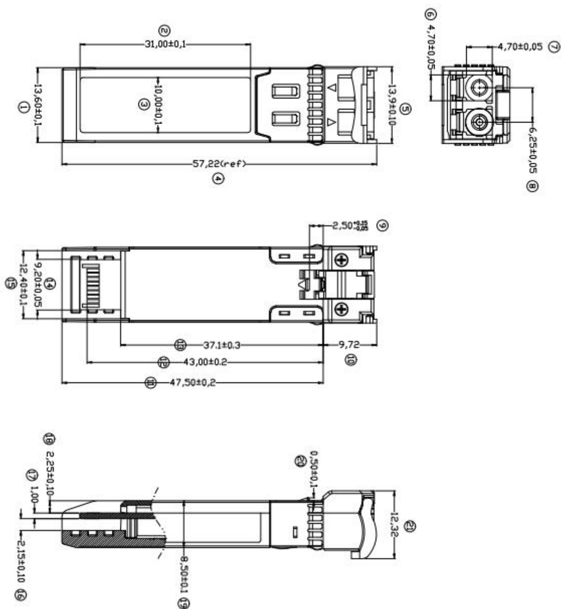
Figure 5, Mechanical Dimensions
