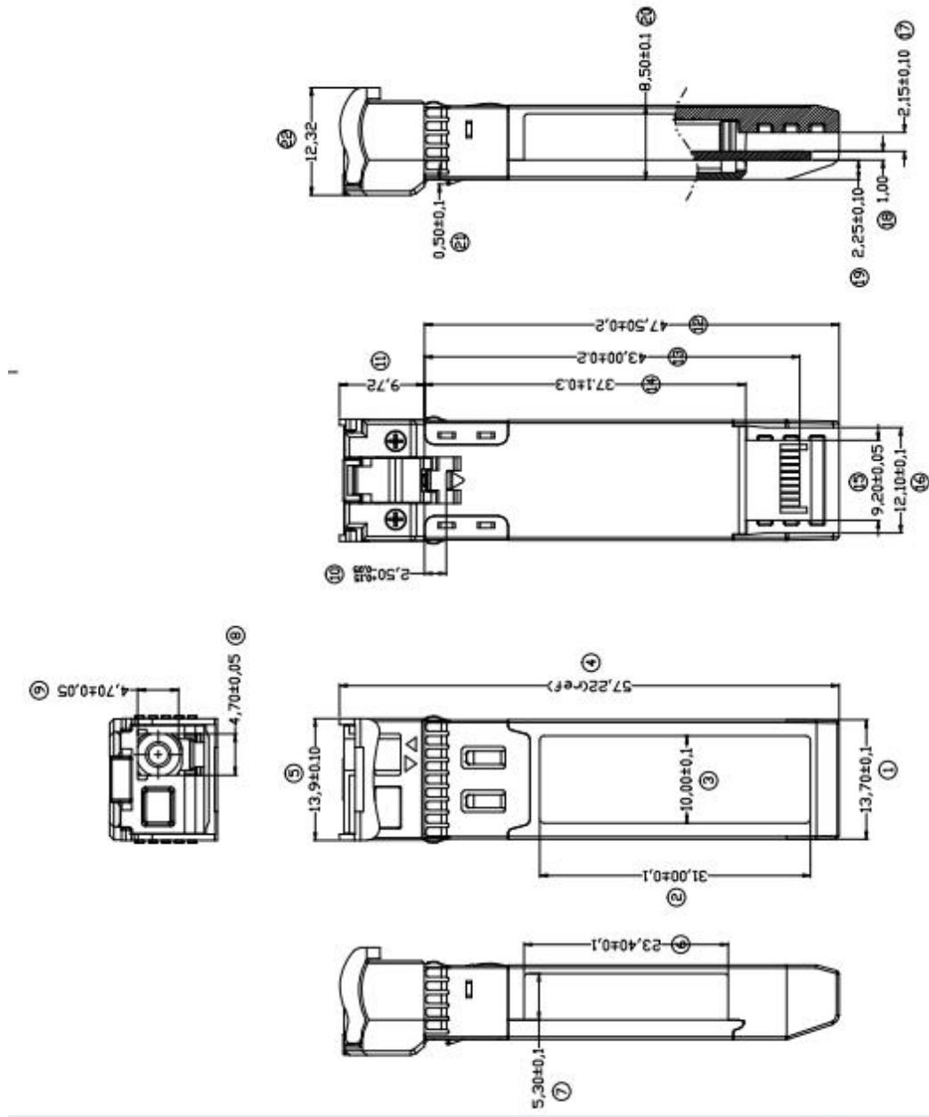
Figure 5, Mechanical Dimensions
