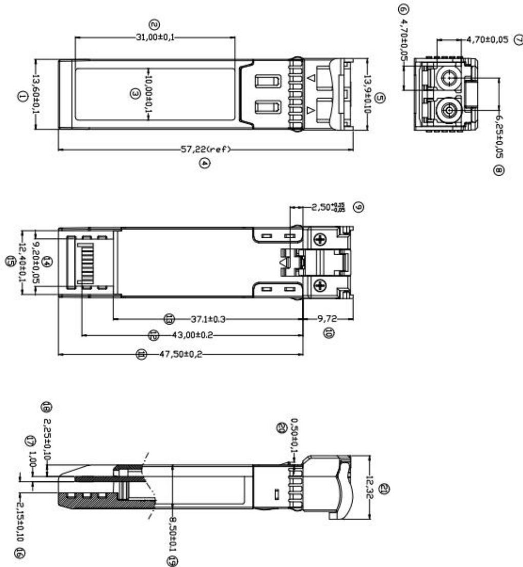
Figure 5, Mechanical Dimensions
