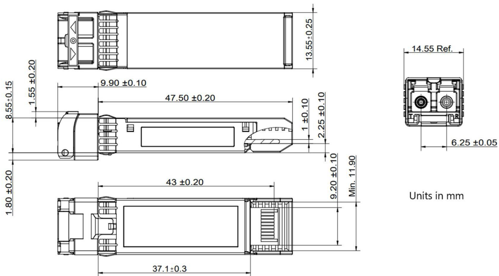
Figure2. Mechanical Outline
