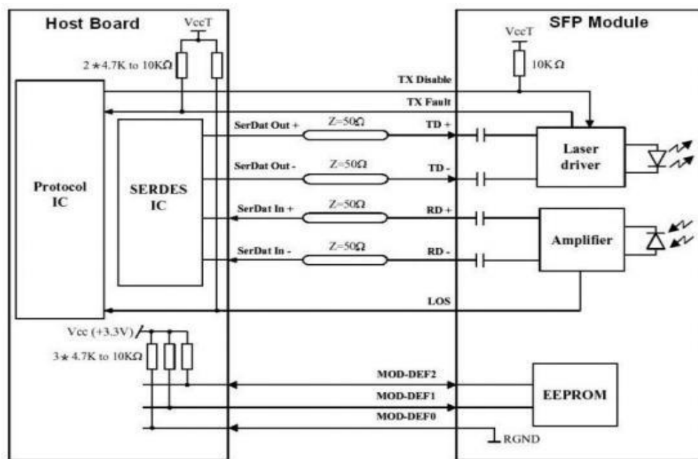
SFP Host Recommended Circuit
