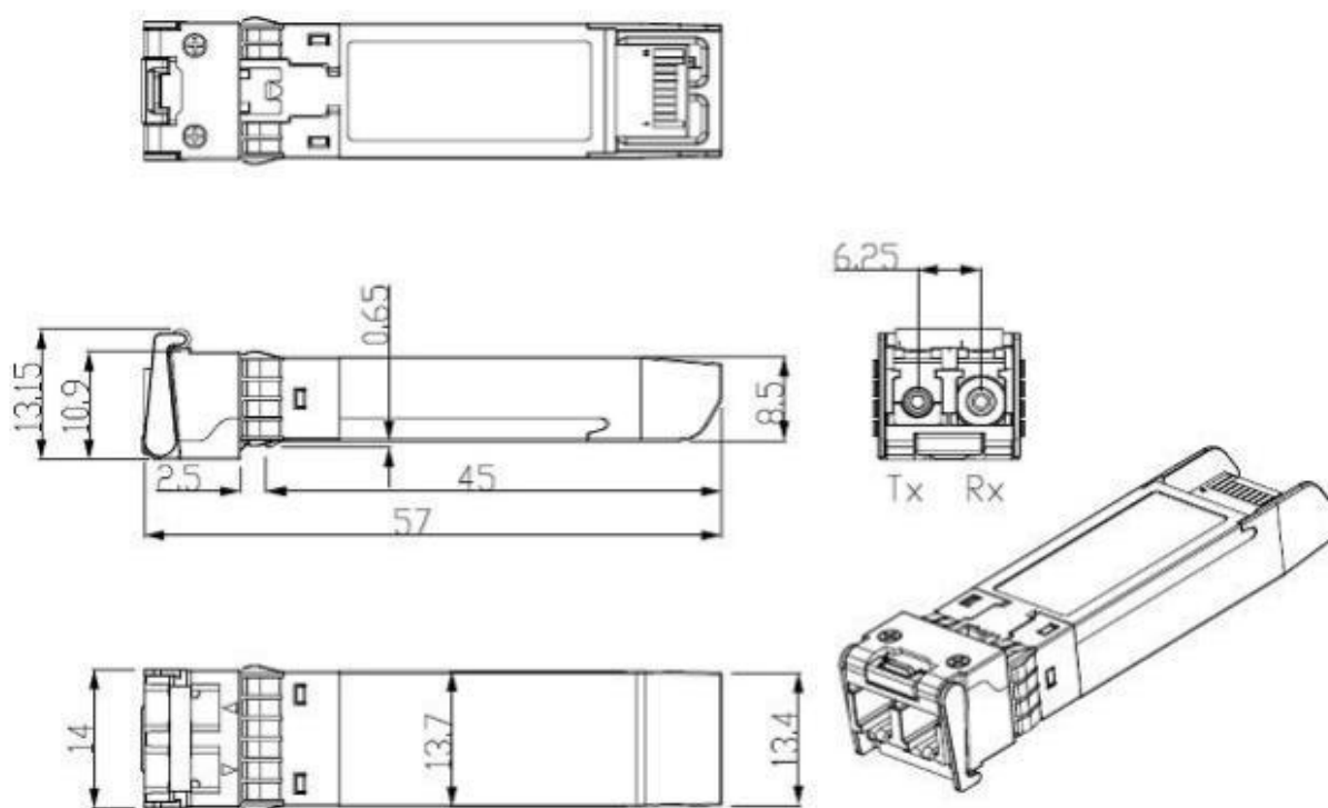
Mechanical Drawing
