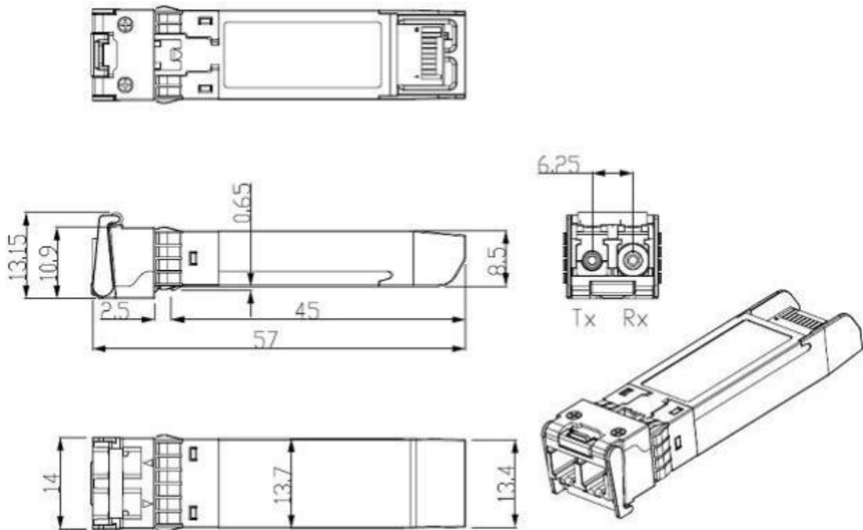
Mechanical Drawing
