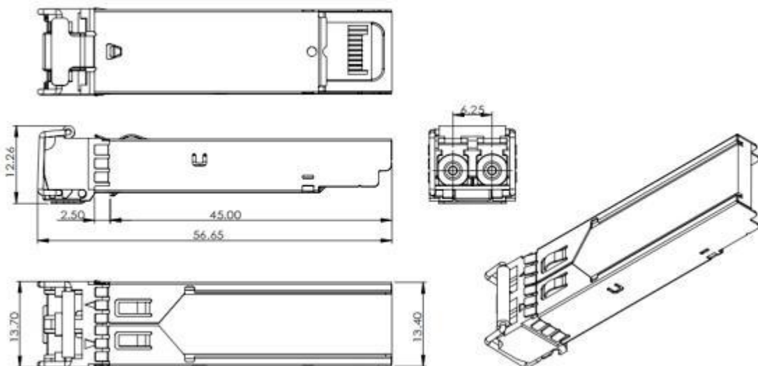
Figure 3. Mechanical Drawing
